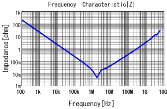
■ GRM31CB31E106KA75 |Z| DCOV, 20degC
