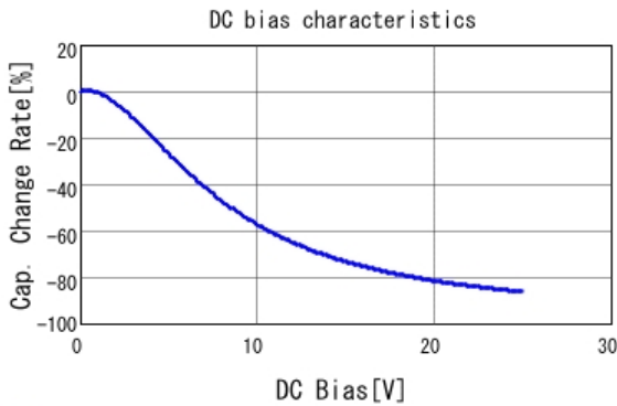
■ GRM31CB31E106KA75 C-DC bias capchange, 20.0degC, AC1.
