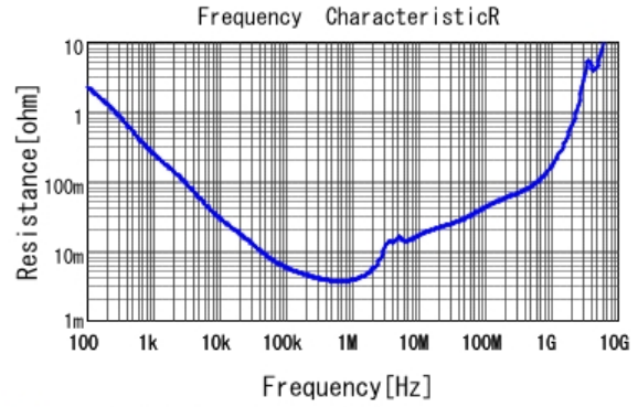
■ GRM31CB31E106KA75 R DCOV, 20degC
