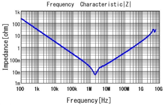
■ GRM31CB31H106KA12 |Z| DCOV, 20degC
