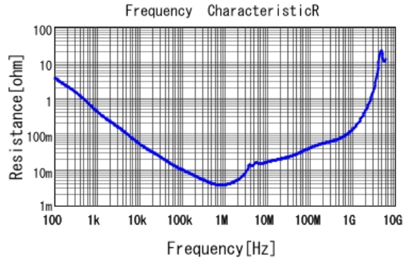
■ GRM31CB31H106KA12 R DCOV, 20degC
