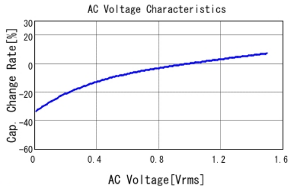
■ GRM31CB31H106KA12 C-AC Voltage capchange, DCOV, 20.0d
