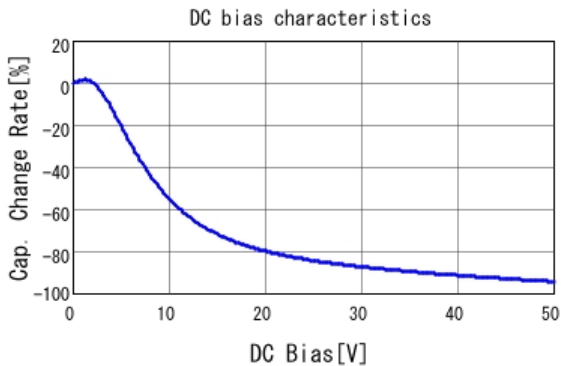
■ GRM31CB31H106KA12 C-DC bias capchange, 20.0degC, AC1.
