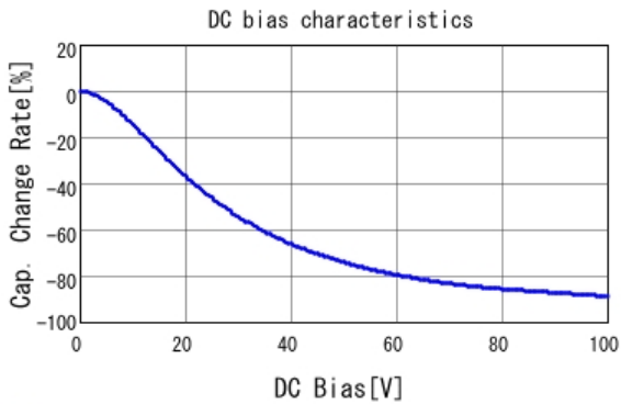
■ GRM31CC72A475KE11 C-DC bias capchange, 25.0degC, AC1V
