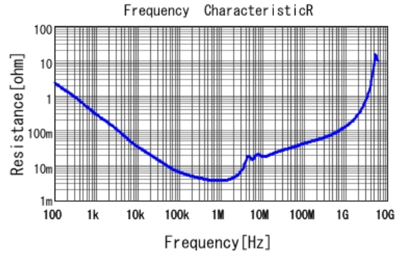
■ GRM31CC72A475KE11 R DCOV, 25degC
