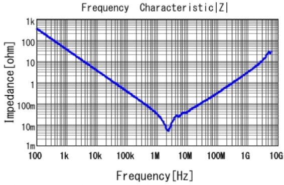
■ GRM31CC72A475KE11 |Z| DCOV, 25degC
