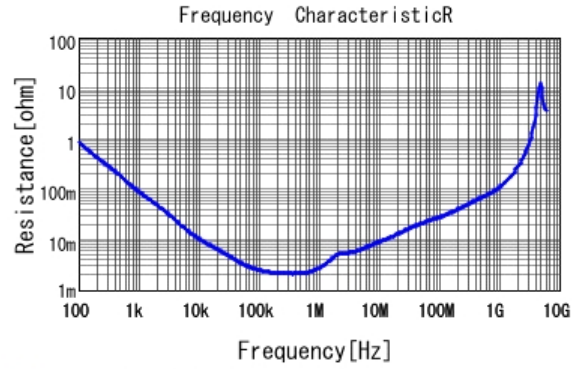
■ GRM31CC81A476ME44 R DCOV, 25degC
