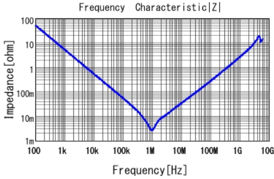
■ GRM31CC81A476ME44 |Z| DCOV, 25degC
