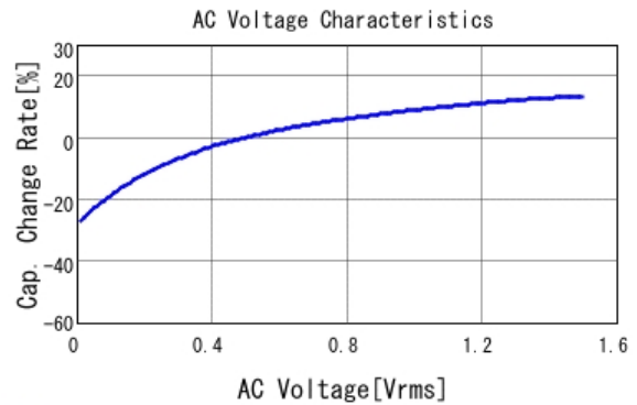
■ GRM31CC81A476ME44 C-AC Voltage capchange, DCOV, 25.0d
