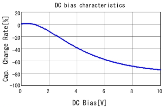
■ GRM31CC81A476ME44 C-DC bias capchange, 25.0degC, ACO.
