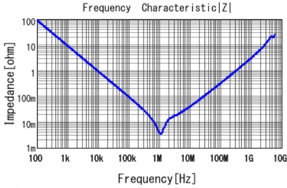
■ GRM31CC81C226ME15 |Z| DCOV, 25degC
