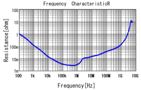
■ GRM31CC81C226ME15 R DCOV, 25degC
