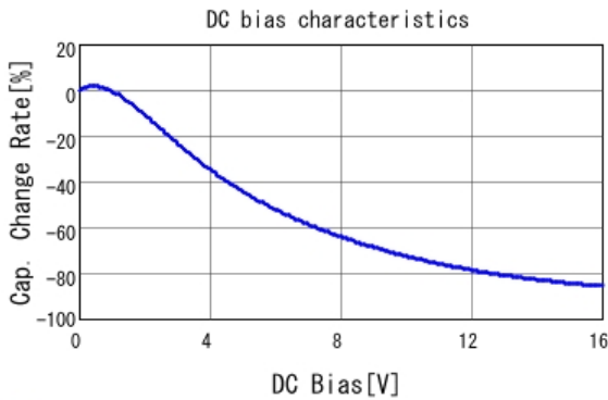
■ GRM31CC81C226ME15 C-DC bias capchange, 25.0degC, AC0.
