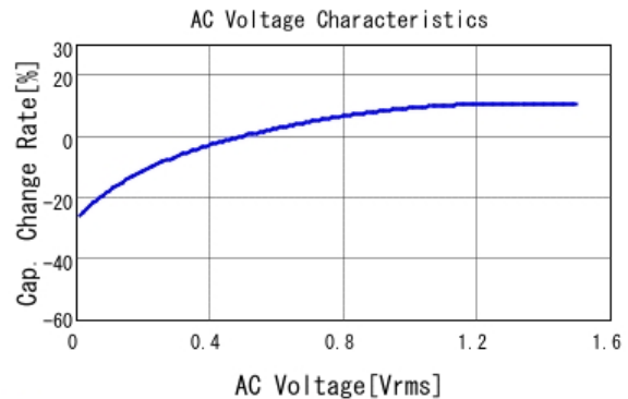
■ GRM31CR60J476ME19 C-AC Voltage capchange, DCOV, 25.0d
