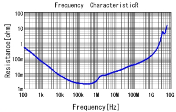
■ GRM31CR60J476ME19 R DCOV, 25degC
