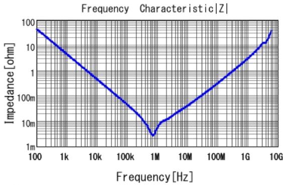
■ GRM31CR60J476ME19 |Z| DCOV, 25degC
