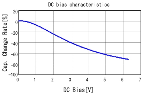
■ GRM31CR60J476ME19 C-DC bias capchange, 25.0degC, AC0.
