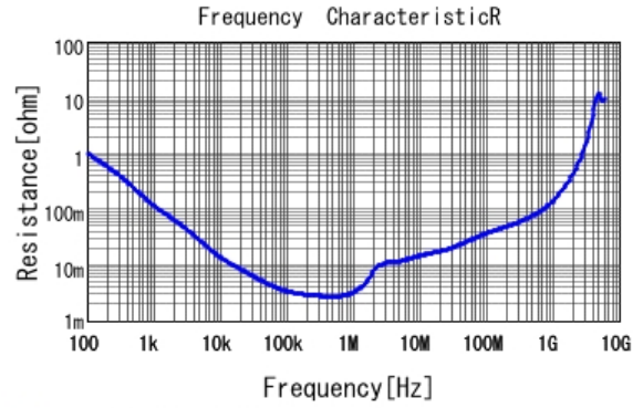
■ GRM31CR61A226KE19 R DCOV, 25degC
