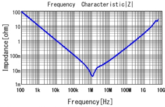
■ GRM31CR61A226KE19 |Z| DCOV, 25degC
