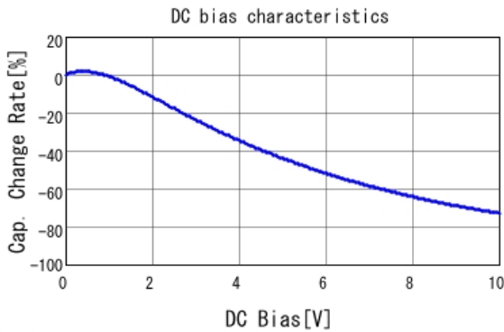
■ GRM31CR61A226KE19 C-DC bias capchange, 25.0degC, AC0.
