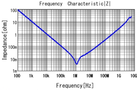
■ GRM31CR61C226KE15 |Z| DCOV, 25degC
