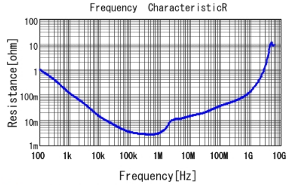
■ GRM31CR61C226KE15 R DCOV, 25degC
