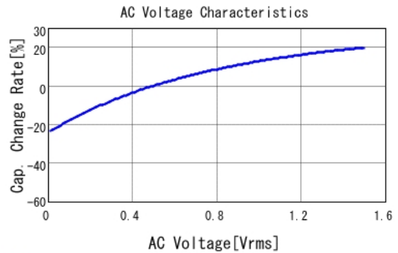
■ GRM31CR61C226KE15 C-AC Voltage capchange, DCOV, 25.0d
