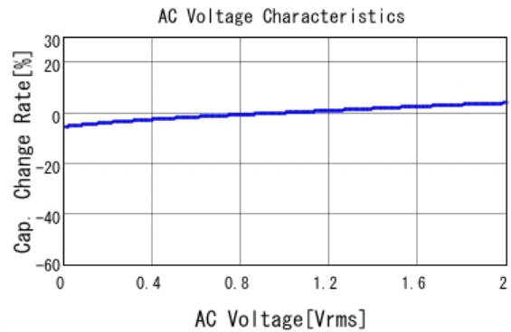
■ GRM31CR61C475KA01 C-AC Voltage capchange, DCOV, 25.0d
