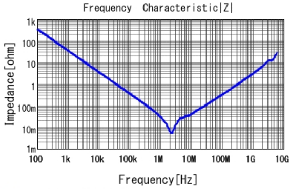
■ GRM31CR61C475KA01 |Z| DCOV, 25degC
