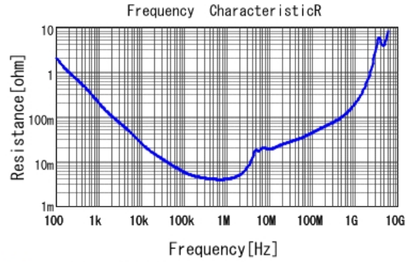
■ GRM31CR61C475KA01 R DCOV, 25degC
