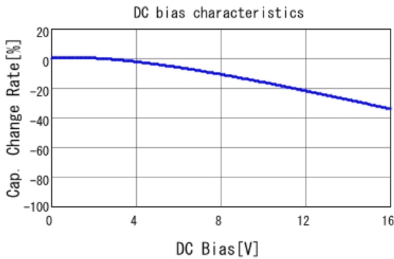
■ GRM31CR61C475KA01 C-DC bias capchange, 25.0degC, AC1.
