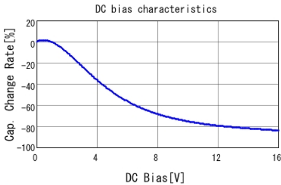
■ GRM31CR61C476ME44 C-DC bias capchange, 25.0degC, AC0.
