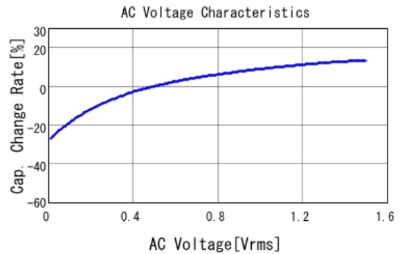
■ GRM31CR61C476ME44 C-AC Voltage capchange, DCOV, 25.0d
