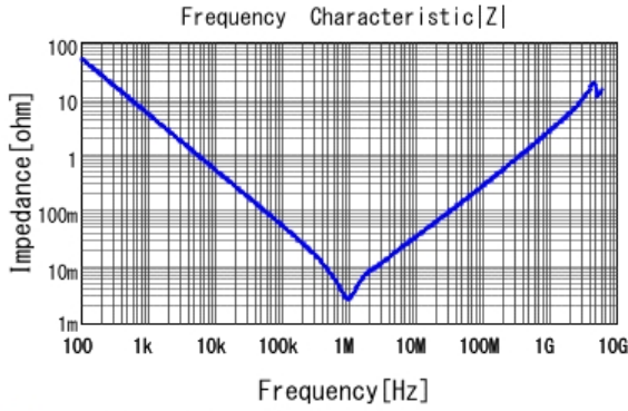
■ GRM31CR61C476ME44 |Z| DCOV, 25degC
