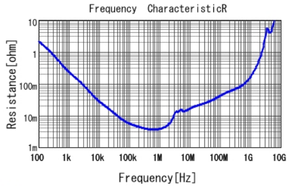
■ GRM31CR61E106KA12 R DCOV, 25degC
