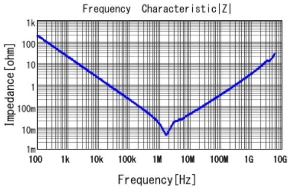
■ GRM31CR61E106KA12 |Z| DCOV, 25degC
