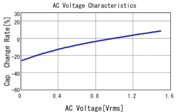
■ GRM31CR61E106KA12 C-AC Voltage capchange, DCOV, 25.0d
