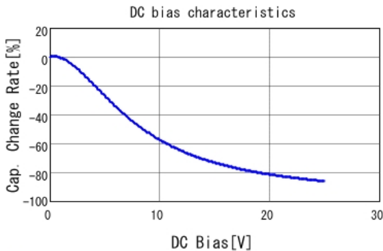
■ GRM31CR61E106KA12 C-DC bias capchange, 25.0degC, AC1.
