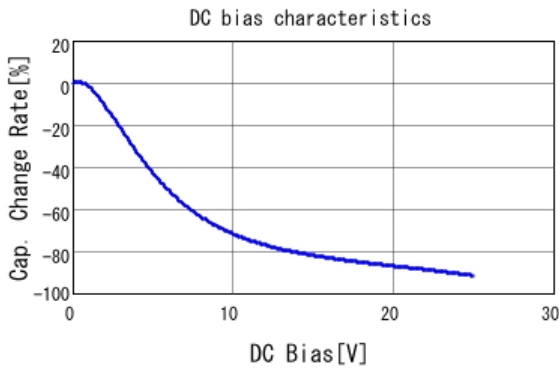
■ GRM31CR61E226KE15 C-DC bias capchange, 25.0degC, AC0.
