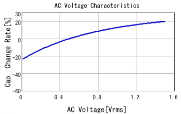
■ GRM31CR61E226KE15 C-AC Voltage capchange, DCOV, 25.0d
