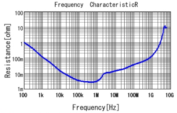
■ GRM31CR61E226KE15 R DCOV, 25degC
