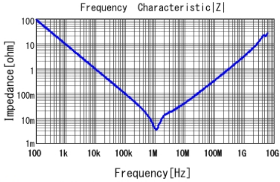
■ GRM31CR61E226KE15 |Z| DCOV, 25degC
