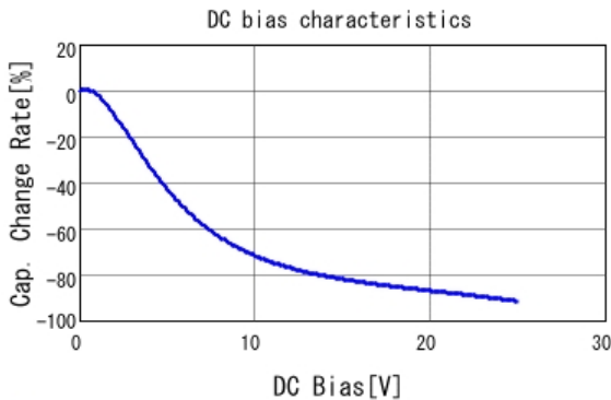
■ GRM31CR61E226ME15 C-DC bias capchange, 25.0degC, AC0.
