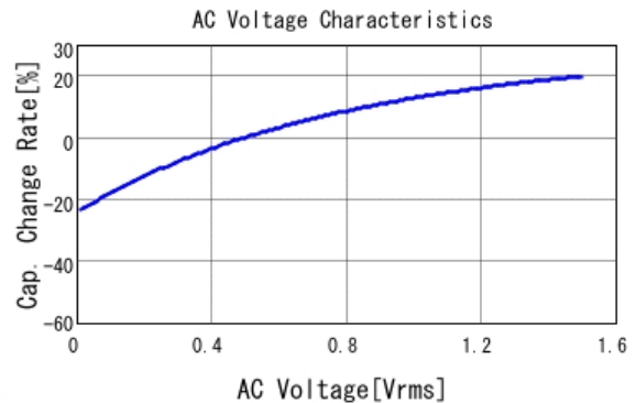
■ GRM31CR61E226ME15 C-AC Voltage capchange, DCOV, 25.0d
