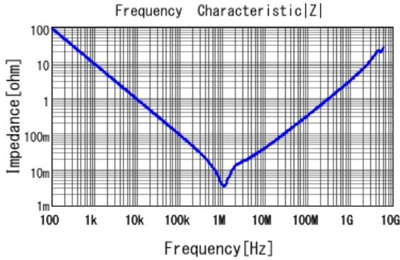
■ GRM31CR61E226ME15 |Z| DCOV, 25degC
