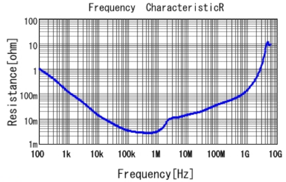
■ GRM31CR61E226ME15 R DCOV, 25degC
