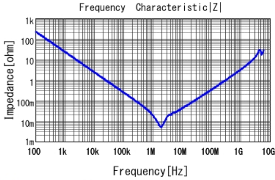
■ GRM31CR61H106KA12 |Z| DCOV, 25degC
