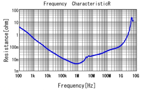
■ GRM31CR61H106KA12 R DCOV, 25degC
