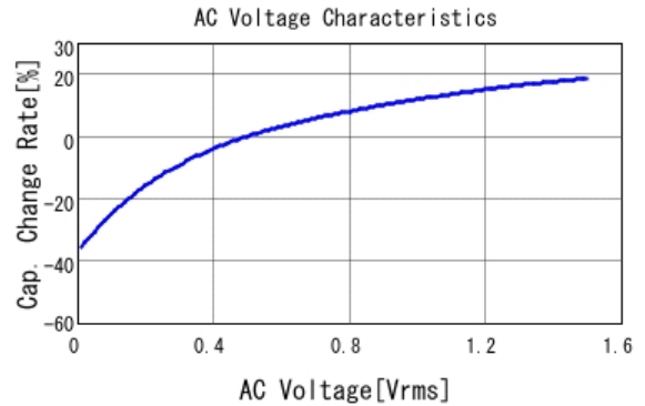
■ GRM31CR71A226KE15 C-AC Voltage capchange, DCOV, 25.0d
