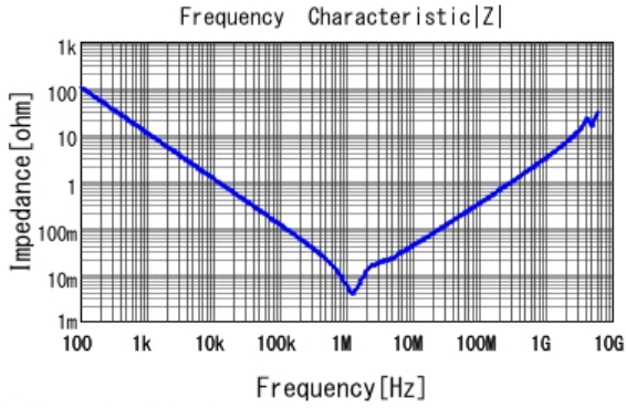
■ GRM31CR71A226KE15 |Z| DCOV, 25degC
