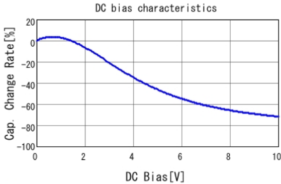
■ GRM31CR71A226KE15 C-DC bias capchange, 25.0degC, AC0.
