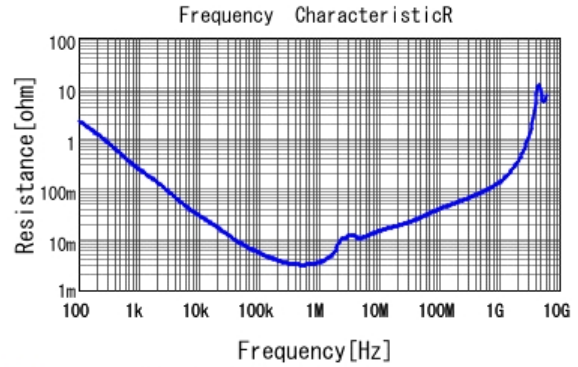
■ GRM31CR71A226ME15 R DCOV, 25degC
