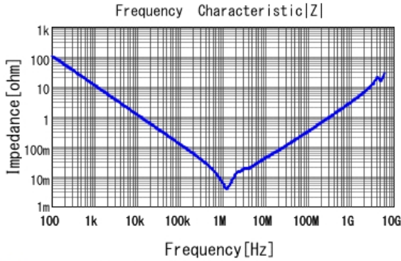
■ GRM31CR71A226ME15 |Z| DCOV, 25degC
