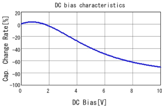
■ GRM31CR71A226ME15 C-DC bias capchange, 25.0degC, AC0.
