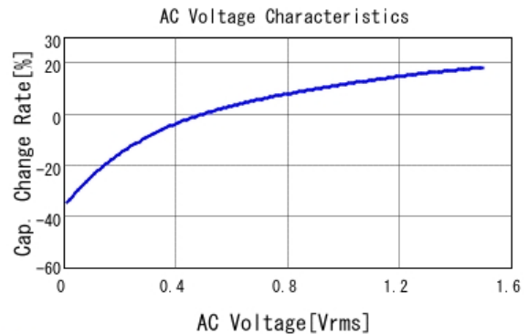
■ GRM31CR71A226ME15 C-AC Voltage capchange, DCOV, 25.0d
