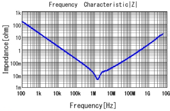
■ GRM31CR71C106KA12 |Z| DCOV, 25degC
