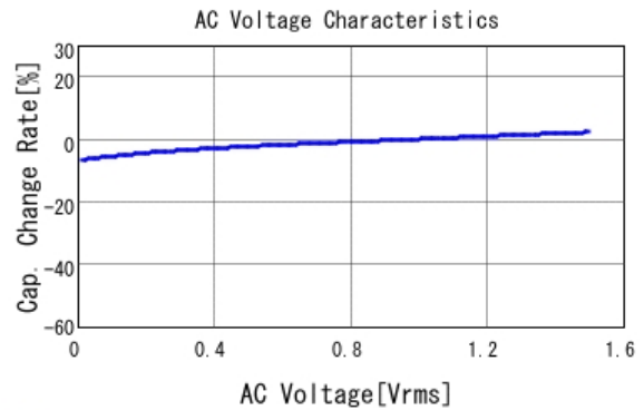
■ GRM31CR71C106KA12 C-AC Voltage capchange, DCOV, 25.0d
