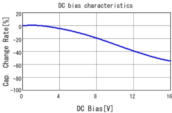
■ GRM31CR71C106KA12 C-DC bias capchange, 25.0degC, AC1.
