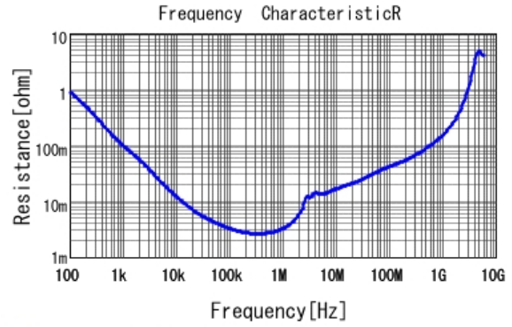
■ GRM31CR71C106KA12 R DCOV, 25degC
