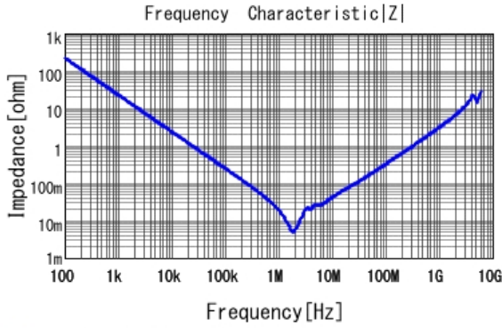
■ GRM31CR71C106KAC7 |Z| DCOV, 25degC
