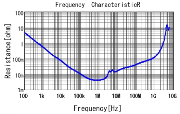
■ GRM31CR71C106KAC7 R DCOV, 25degC
