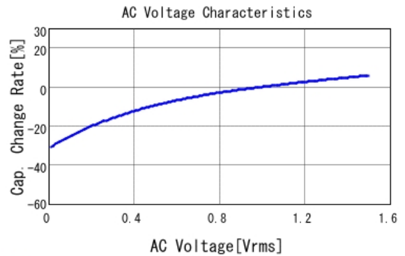
■ GRM31CR71C106KAC7 C-AC Voltage capchange, DCOV, 25.0d
