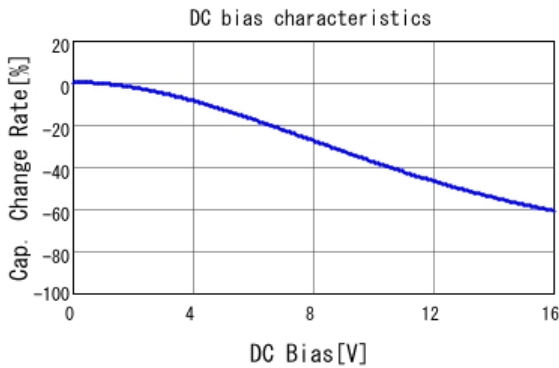
■ GRM31CR71C106KAC7 C-DC bias capchange, 25.0degC, AC1.
