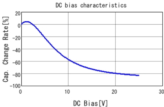
■ GRM31CR71E106KA12 C-DC bias capchange, 25.0degC, AC1.
