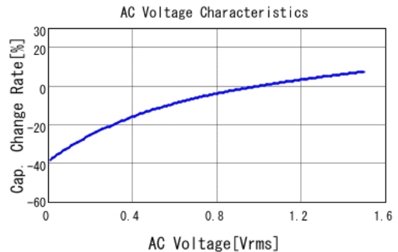
■ GRM31CR71E106KA12 C-AC Voltage capchange, DCOV, 25.0d
