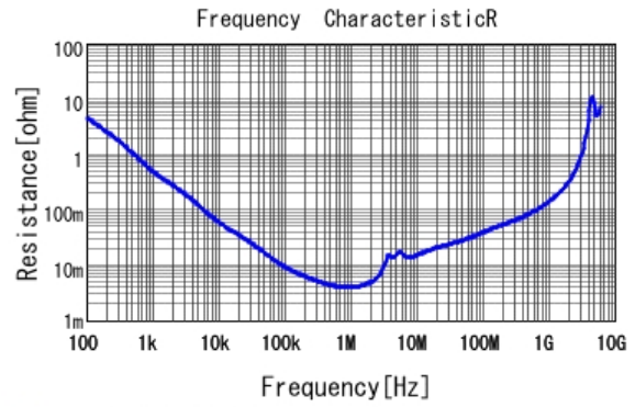
■ GRM31CR71E106KA12 R DCOV, 25degC
