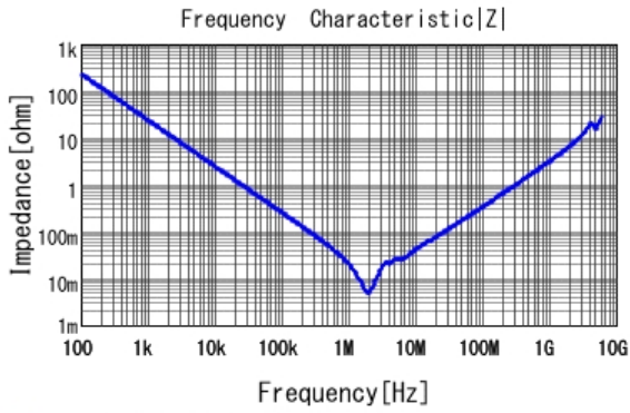
■ GRM31CR71E106KA12 |Z| DCOV, 25degC
