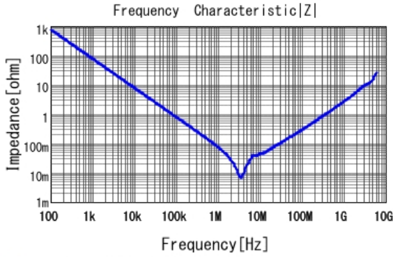
■ GRM31CR71H225KA88 |Z| DCOV, 25degC
