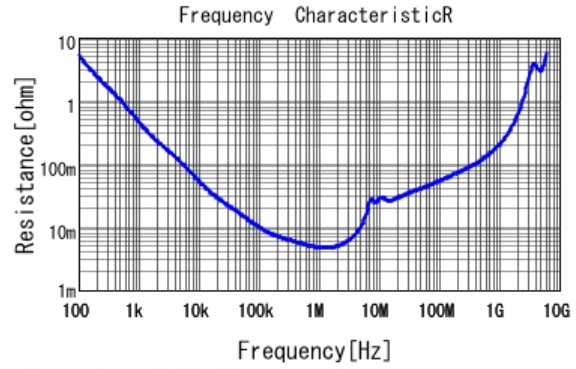
■ GRM31CR71H225KA88 R DCOV, 25degC
