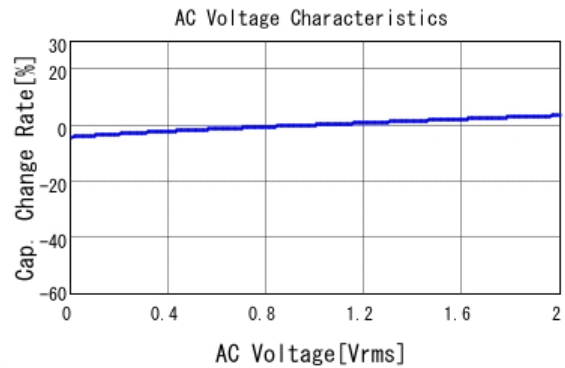
■ GRM31CR71H225KA88 C-AC Voltage capchange, DCOV, 25.0d
