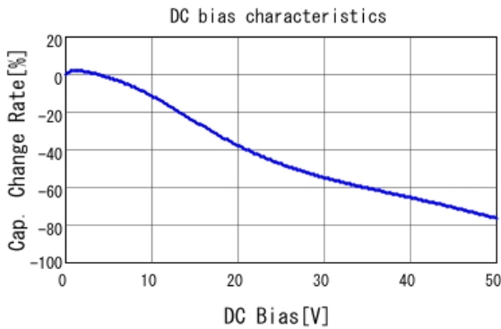
■ GRM31CR71H475KA12 C-DC bias capchange, 25.0degC, AC1.
