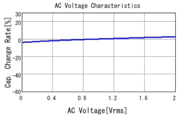
■ GRM31CR71H475KA12 C-AC Voltage capchange, DCOV, 25.0d
