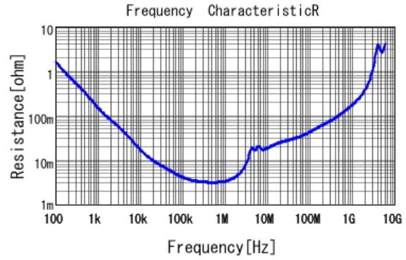
■ GRM31CR71H475KA12 R DCOV, 25degC
