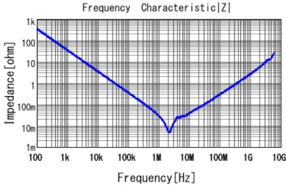
■ GRM31CR71H475KA12 |Z| DCOV, 25degC
