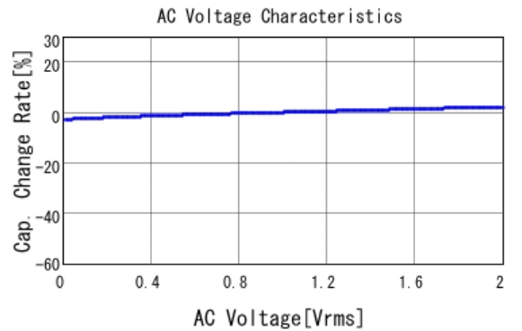
■ GRM31CR72A105KA01 C-AC Voltage capchange, DCOV, 25.0d
