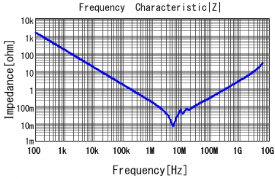
■ GRM31CR72A105KA01 |Z| DCOV, 25degC
