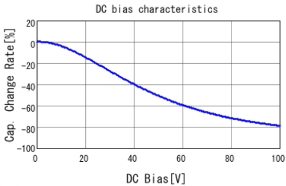
■ GRM31CR72A105KA01 C-DC bias capchange, 25.0degC, AC1.
