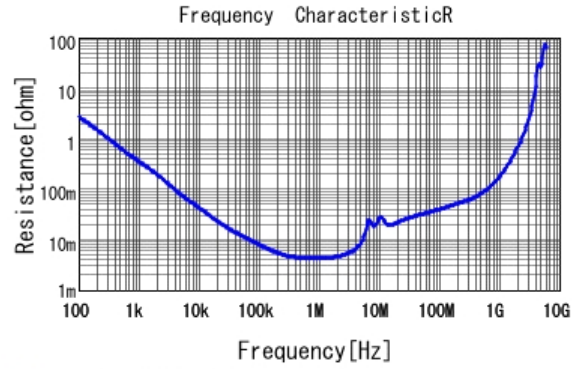
■ GRM31CR72A225KA73 R DCOV, 25degC
