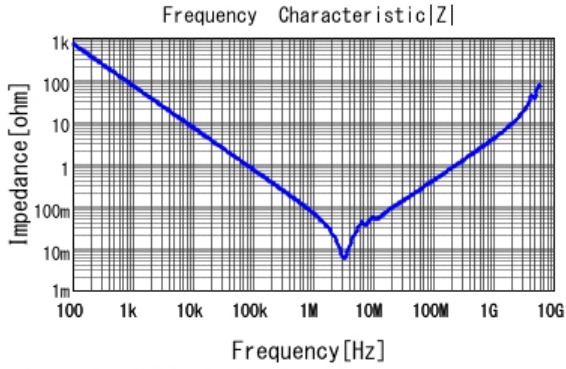
■ GRM31CR72A225KA73 |Z| DCOV, 25degC
