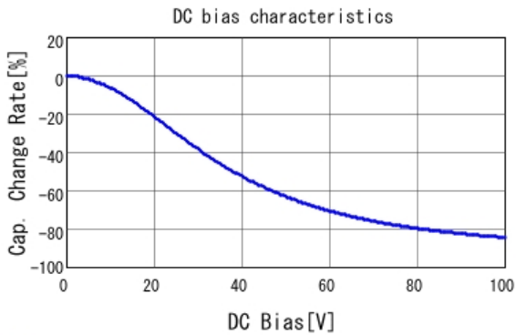
■ GRM31CR72A225KA73 C-DC bias capchange, 25.0degC, AC1.
