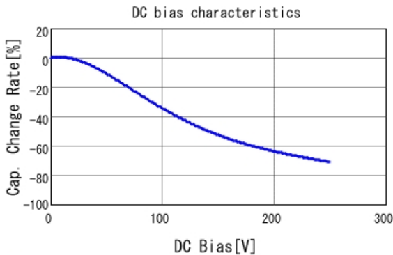
■ GRM31CR72E333KW03 C-DC bias capchange, 25.0degC, AC1V
