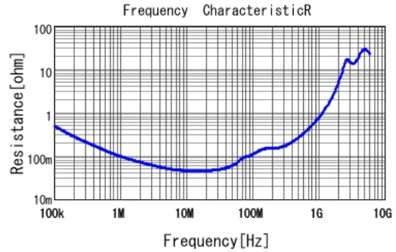
■ GRM31CR72E333KW03 R DCOV, 25degC
