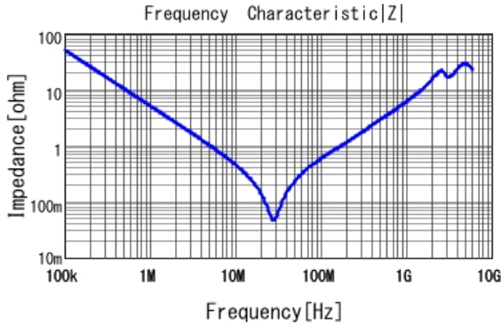
■ GRM31CR72E333KW03 |Z| DCOV, 25degC
