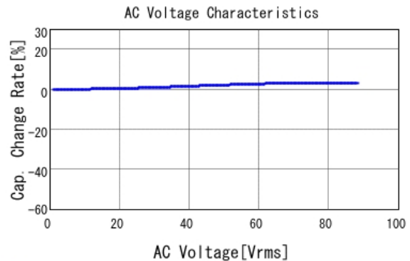
■ GRM31CR72E333KW03 C-AC Voltage capchange, DCOV, 25.0d
