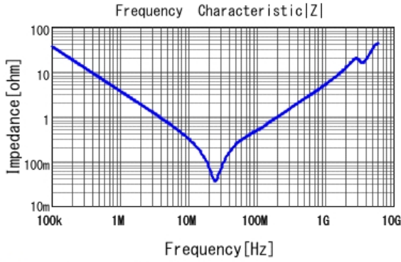
■ GRM31CR72E473KW03 |Z| DCOV, 25degC
