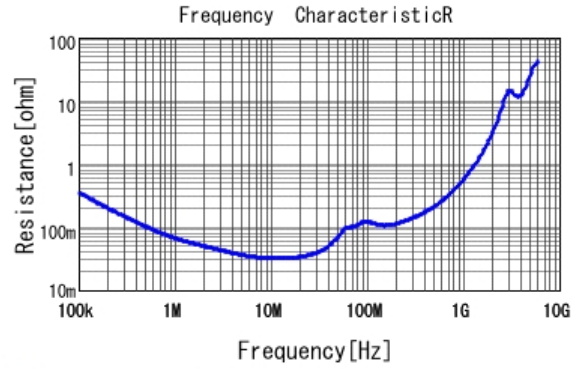
■ GRM31CR72E473KW03 R DCOV, 25degC
