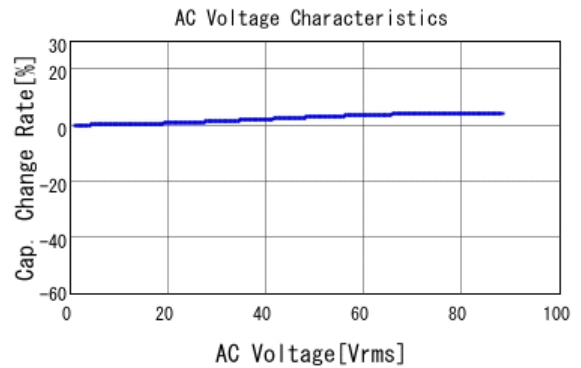
■ GRM31CR72E473KW03 C-AC Voltage capchange, DCOV, 25.0d
