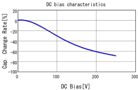
■ GRM31CR72E473KW03 C-DC bias capchange, 25.0degC, AC1V
