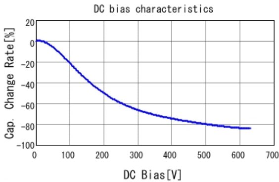
■ GRM31CR72J153KW03 C-DC bias capchange, 25.0degC, AC1V
