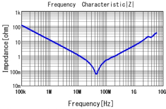
■ GRM31CR72J153KW03 |Z| DCOV, 25degC
