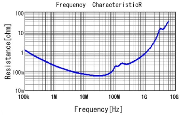
■ GRM31CR72J153KW03 R DCOV, 25degC
