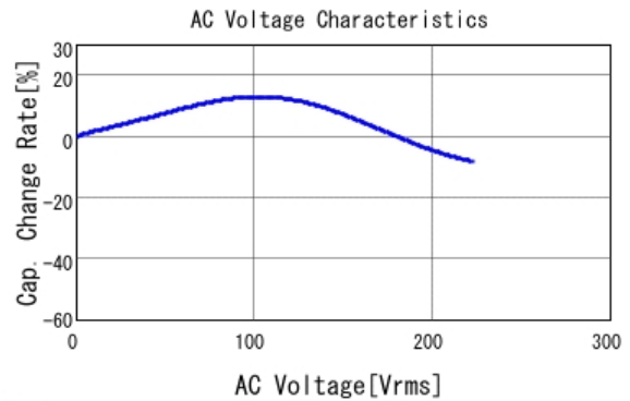
■ GRM31CR72J153KW03 C-AC Voltage capchange, DCOV, 25.0d
