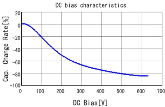
■ GRM31CR72J223KW03 C-DC bias capchange, 25.0degC, AC1V
