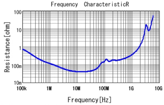
■ GRM31CR72J223KW03 R DCOV, 25degC
