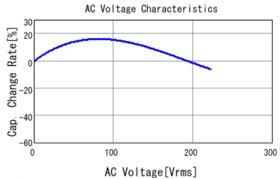
■ GRM31CR72J223KW03 C-AC Voltage capchange, DCOV, 25.0d
