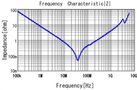
■ GRM31CR72J223KW03 |Z| DCOV, 25degC
