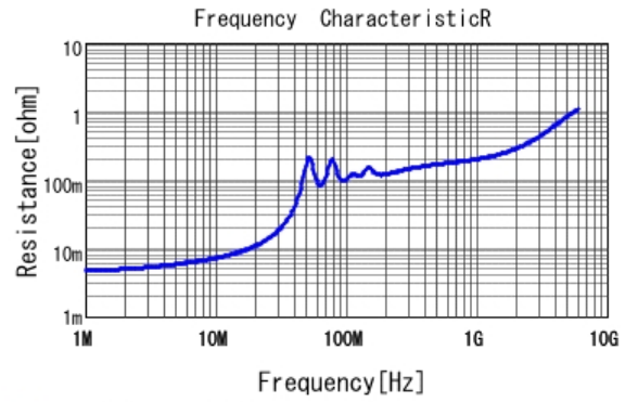
■ GRM31M5C1H473JA01 R DCOV, 25degC
