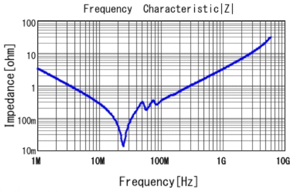
■ GRM31M5C1H473JA01 |Z| DCOV, 25degC
