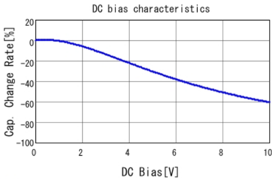
■ GRM31MB31A106KE18 C-DC bias capchange, 20.0degC, AC1.
