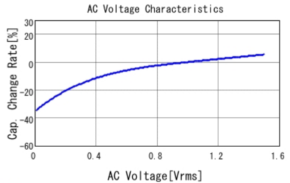
■ GRM31MB31A106KE18 C-AC Voltage capchange, DCOV, 20.0d
