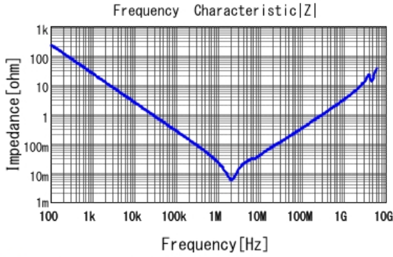
■ GRM31MB31A106KE18 |Z| DCOV, 20degC
