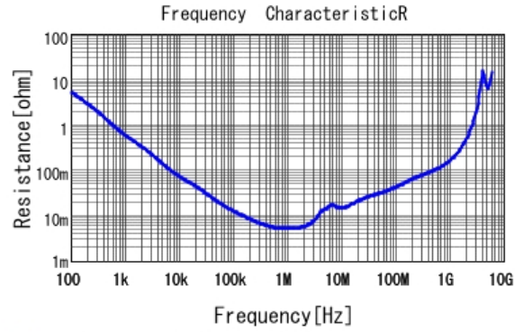
■ GRM31MB31A106KE18 R DCOV, 20degC
