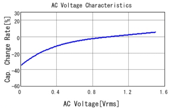
■ GRM31MR61A106KE19 C-AC Voltage capchange, DCOV, 25.0d
