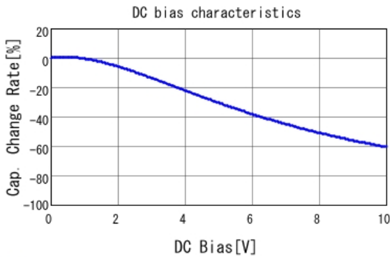
■ GRM31MR61A106KE19 C-DC bias capchange, 25.0degC, AC1.
