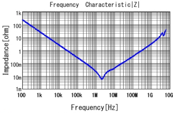
■ GRM31MR61A106KE19 |Z| DCOV, 25degC
