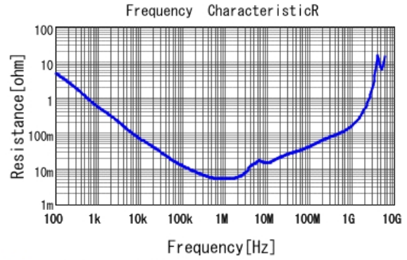
■ GRM31MR61A106KE19 R DCOV, 25degC
