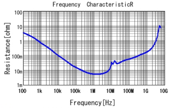
■ GRM31MR61C105KA01 R DCOV, 25degC
