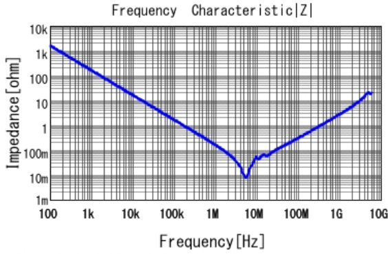
■ GRM31MR61C105KA01 |Z| DCOV, 25degC
