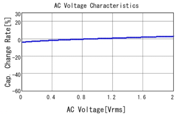
■ GRM31MR71C105KA01 C-AC Voltage capchange, DCOV, 25.0d
