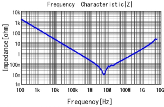
■ GRM31MR71C105KA01 |Z| DCOV, 25degC
