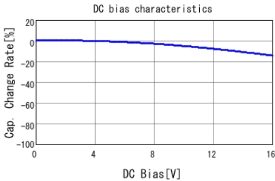
■ GRM31MR71C105KA01 C-DC bias capchange, 25.0degC, AC1.
