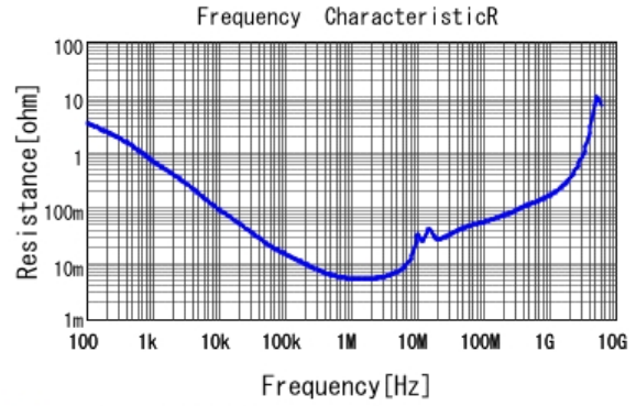
■ GRM31MR71C105KA01 R DCOV, 25degC
