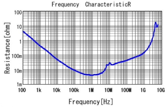
■ GRM31MR71C225MA35 R DCOV, 25degC
