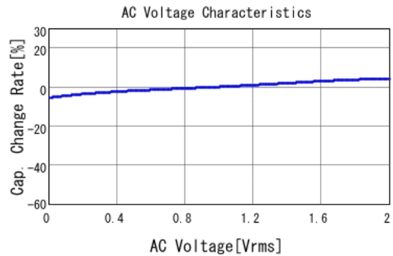
■ GRM31MR71C225MA35 C-AC Voltage capchange, DCOV, 25.0d
