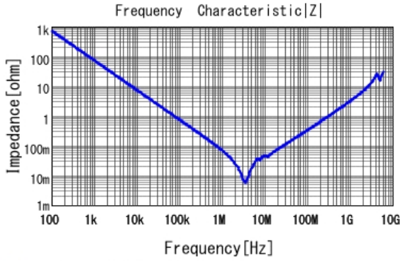
■ GRM31MR71C225MA35 |Z| DCOV, 25degC
