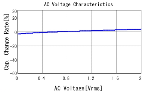
■ GRM31MR71E105KA01 C-AC Voltage capchange, DCOV, 25.0d
