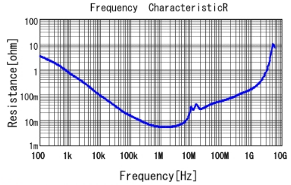
■ GRM31MR71E105KA01 R DCOV, 25degC
