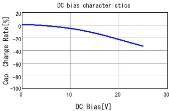
■ GRM31MR71E105KA01 C-DC bias capchange, 25.0degC, AC1.
