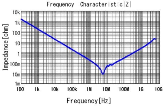
■ GRM31MR71E105KA01 |Z| DCOV, 25degC
