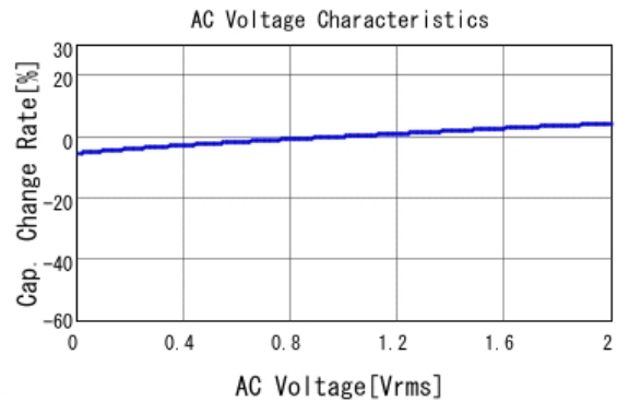
■ GRM31MR71E225KA93 C-AC Voltage capchange, DCOV, 25.0d
