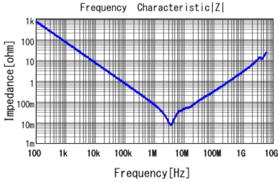
■ GRM31MR71E225KA93 |Z| DCOV, 25degC
