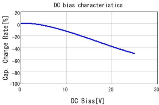
■ GRM31MR71E225KA93 C-DC bias capchange, 25.0degC, AC1.
