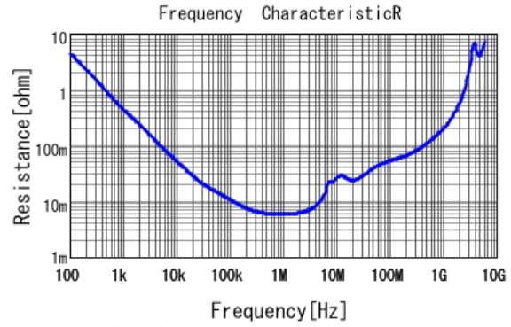
■ GRM31MR71E225KA93 R DCOV, 25degC
