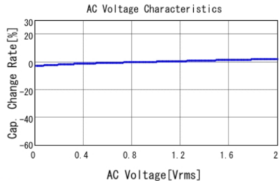
■ GRM31MR71H224KA01 C-AC Voltage capchange, DCOV, 25.0d
