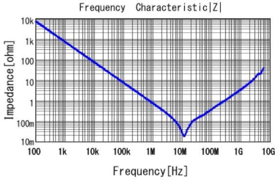
■ GRM31MR71H224KA01 |Z| DCOV, 25degC
