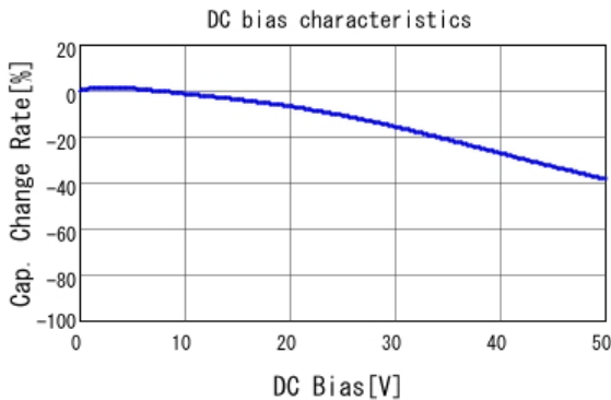
■ GRM31MR71H224KA01 C-DC bias capchange, 25.0degC, AC1.
