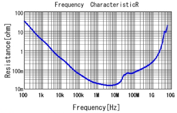
■ GRM31MR71H224KA01 R DCOV, 25degC
