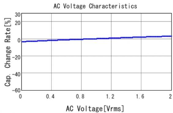
■ GRM31MR71H474KA01 C-AC Voltage capchange, DCOV, 25.0d
