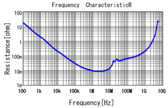
■ GRM31MR71H474KA01 R DCOV, 25degC
