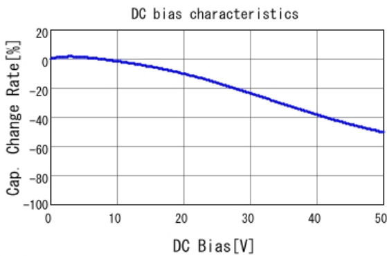
■ GRM31MR71H474KA01 C-DC bias capchange, 25.0degC, AC1.
