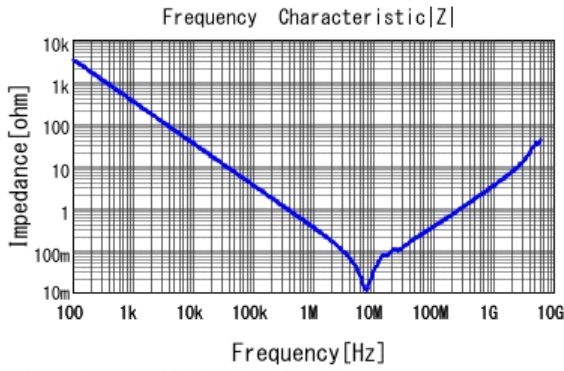
■ GRM31MR71H474KA01 |Z| DCOV, 25degC
