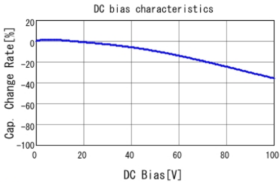
■ GRM31MR72A473KA01 C-DC bias capchange, 25.0degC, AC1.
