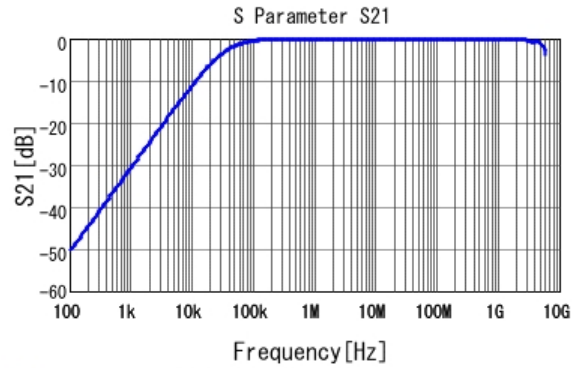
■ GRM31MR72A473KA01 S21 DC0V, 25degC
