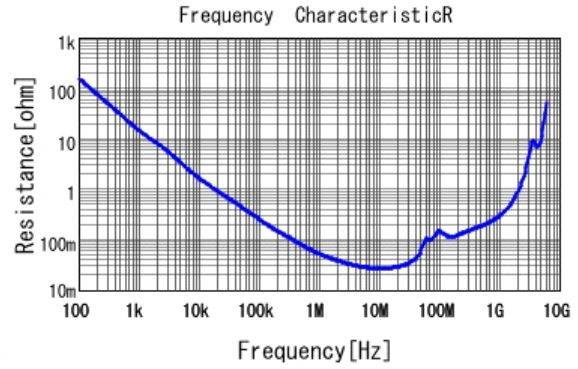
■ GRM31MR72A473KA01 R DCOV, 25degC
