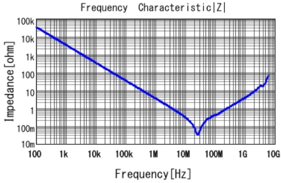
■ GRM31MR72A473KA01 |Z| DCOV, 25degC
