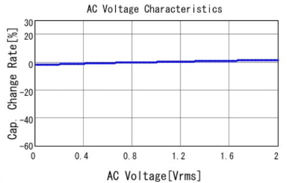
■ GRM31MR72A473KA01 C-AC Voltage capchange, DCOV, 25.0d
