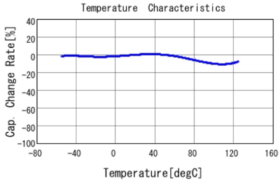
■ GRM31MR72A473KA01 C-Temp. capchange, DC0.0V, AC1.0V rm
