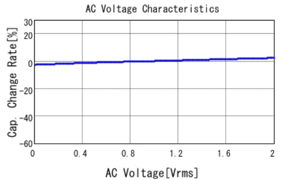
■ GRM31MR72A474KA35 C-AC Voltage capchange, DCOV, 25.0d
