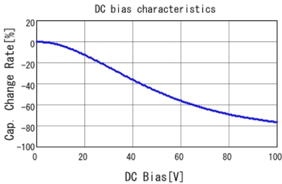
■ GRM31MR72A474KA35 C-DC bias capchange, 25.0degC, AC1.
