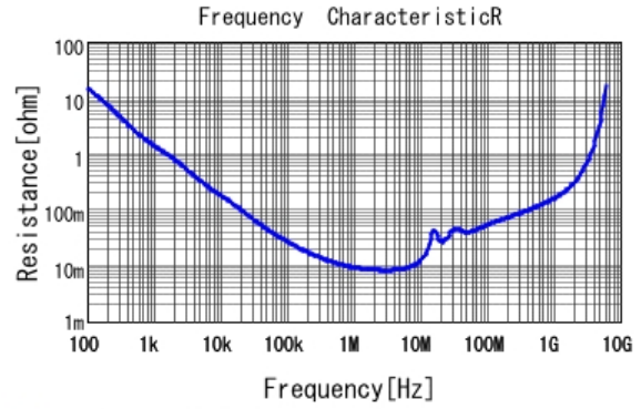
■ GRM31MR72A474KA35 R DCOV, 25degC
