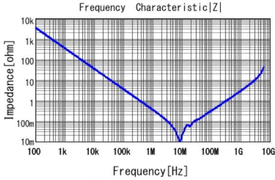
■ GRM31MR72A474KA35 |Z| DCOV, 25degC
