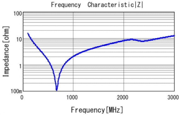
■ GRM32A7U3D101JW31 |Z| DCOV, 25degC
