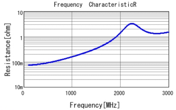
■ GRM32A7U3D101JW31 R DCOV, 25degC
