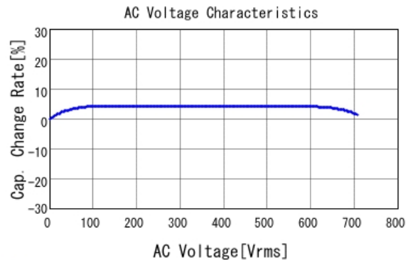
■ GRM32A7U3D101JW31 C-AC Voltage capchange, DCOV, 25.0d
