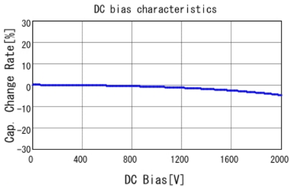
■ GRM32B7U3D221JW31 C-DC bias capchange, 25.0degC, AC1V
