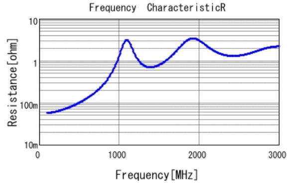
■ GRM32B7U3D221JW31 R DCOV, 25degC
