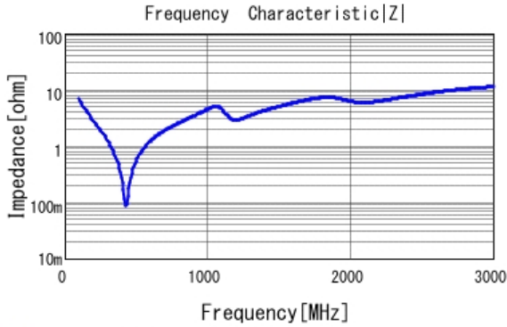
■ GRM32B7U3D221JW31 |Z| DCOV, 25degC
