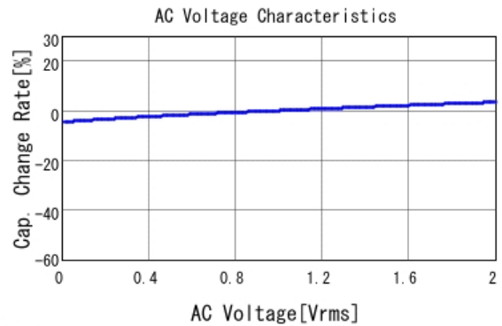
■ GRM32DB11E475KA61 C-AC Voltage capchange, DCOV, 20.0d
