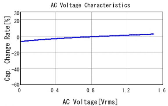
■ GRM32DR61C106KA01 C-AC Voltage capchange, DCOV, 25.0d
