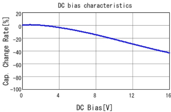
■ GRM32DR61C106KA01 C-DC bias capchange, 25.0degC, AC1.
