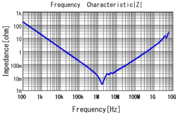
■ GRM32DR61C106KA01 |Z| DCOV, 25degC
