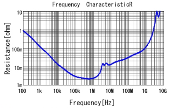
■ GRM32DR61C106KA01 R DCOV, 25degC
