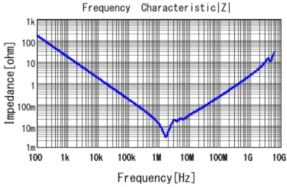
■ GRM32DR71A106KA01 |Z| DCOV, 25degC
