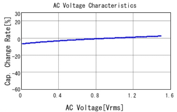
■ GRM32DR71A106KA01 C-AC Voltage capchange, DCOV, 25.0d
