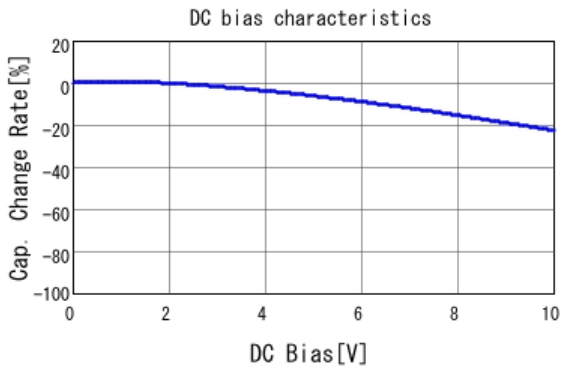
■ GRM32DR71A106KA01 C-DC bias capchange, 25.0degC, AC1.
