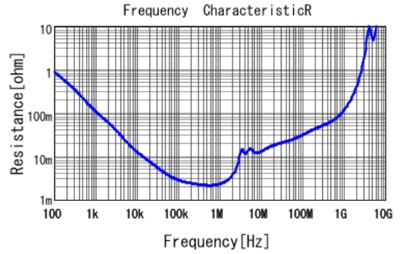
■ GRM32DR71A106KA01 R DCOV, 25degC
