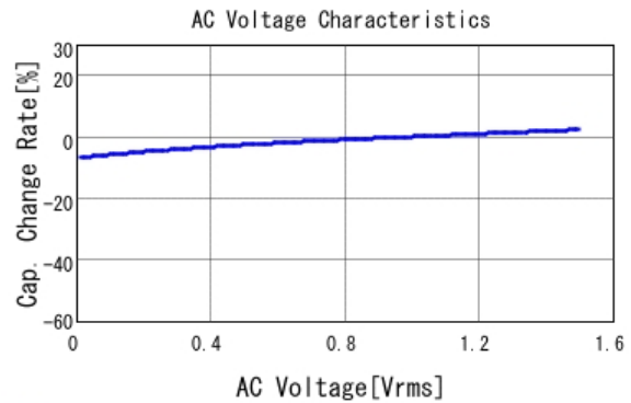
■ GRM32DR71C106KA01 C-AC Voltage capchange, DCOV, 25.0d
