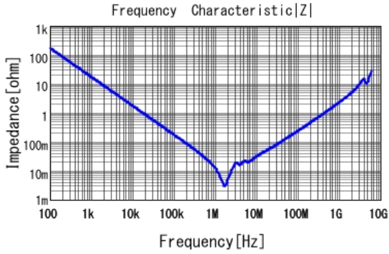
■ GRM32DR71C106KA01 |Z| DCOV, 25degC
