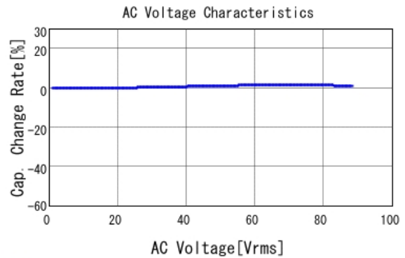
■ GRM32DR72E104KW01 C-AC Voltage capchange, DCOV, 25.0d
