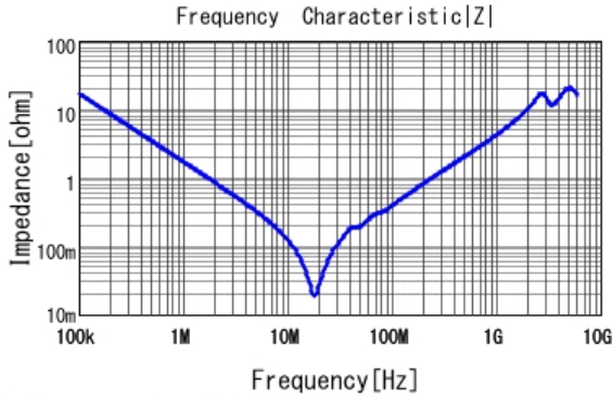
■ GRM32DR72E104KW01 |Z| DCOV, 25degC
