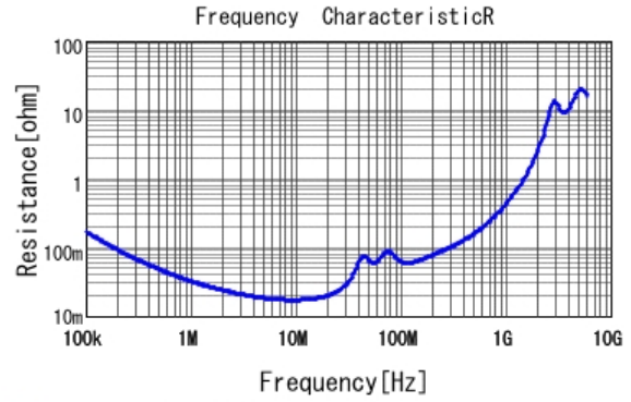
■ GRM32DR72E104KW01 R DCOV, 25degC
