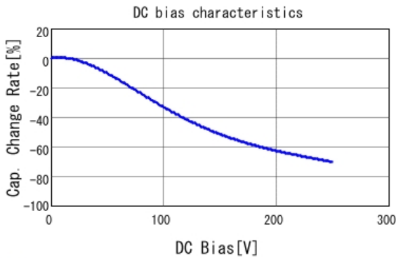
■ GRM32DR72E104KW01 C-DC bias capchange, 25.0degC, AC1V
