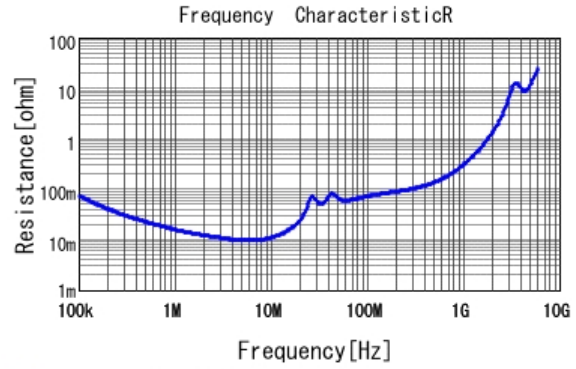
■ GRM32DR72E224KW01 R DC0V, 25degC
