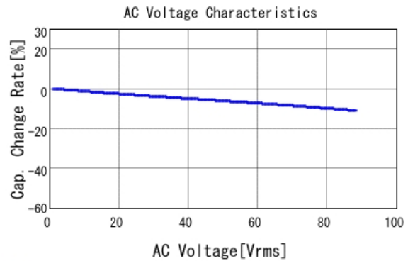
■ GRM32DR72E224KW01 C-AC Voltage capchange, DC0V, 25.0d
