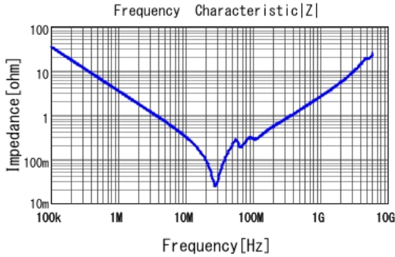
■ GRM32DR72J473KW01 |Z| DCOV, 25degC
