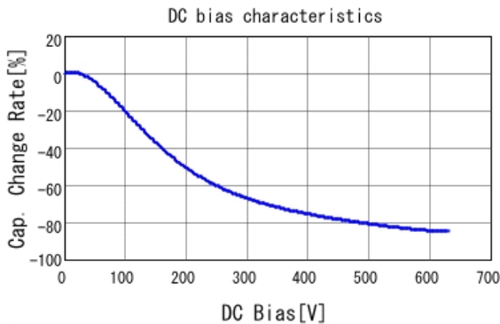
■ GRM32DR72J473KW01 C-DC bias capchange, 25.0degC, AC1V
