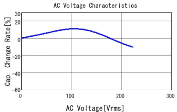
■ GRM32DR72J473KW01 C-AC Voltage capchange, DCOV, 25.0d
