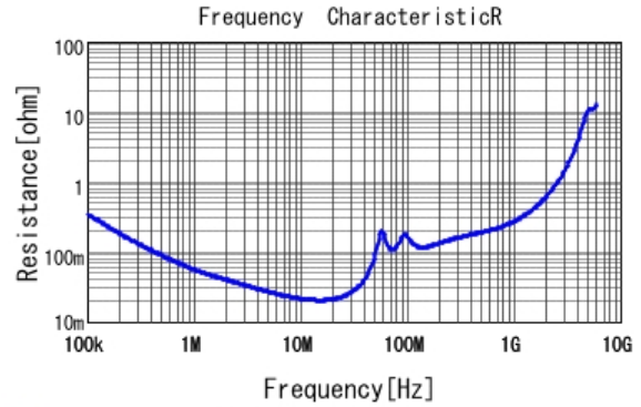
■ GRM32DR72J473KW01 R DCOV, 25degC
