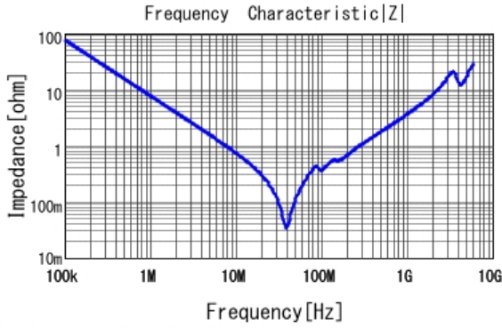
■ GRM32DR73A223KW01 |Z| DCOV, 25degC
