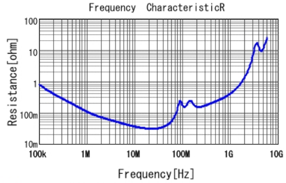
■ GRM32DR73A223KW01 R DCOV, 25degC
