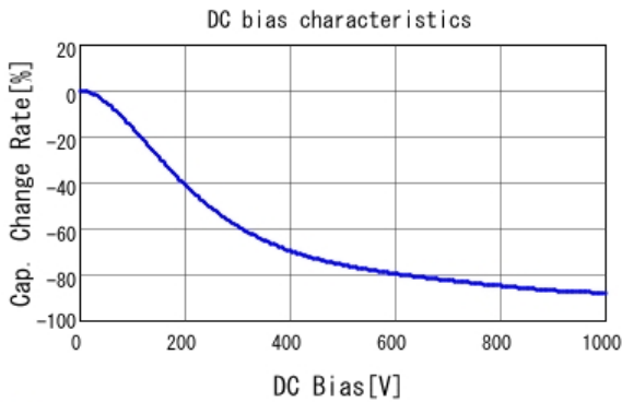
■ GRM32DR73A223KW01 C-DC bias capchange, 25.0degC, AC1V
