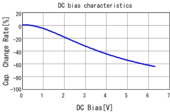
■ GRM32EB30J107ME16 C-DC bias capchange, 20.0degC, AC0.
