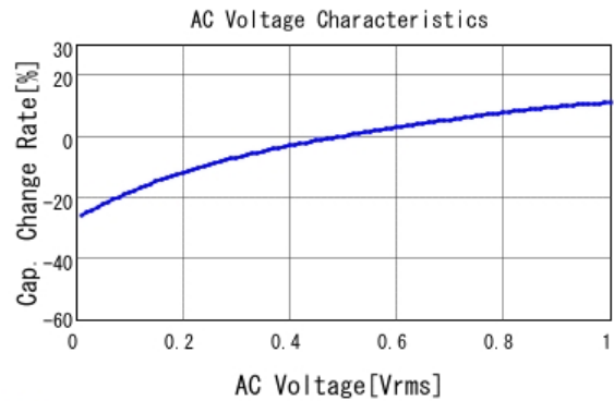
■ GRM32EB30J107ME16 C-AC Voltage capchange, DCOV, 20.0d
